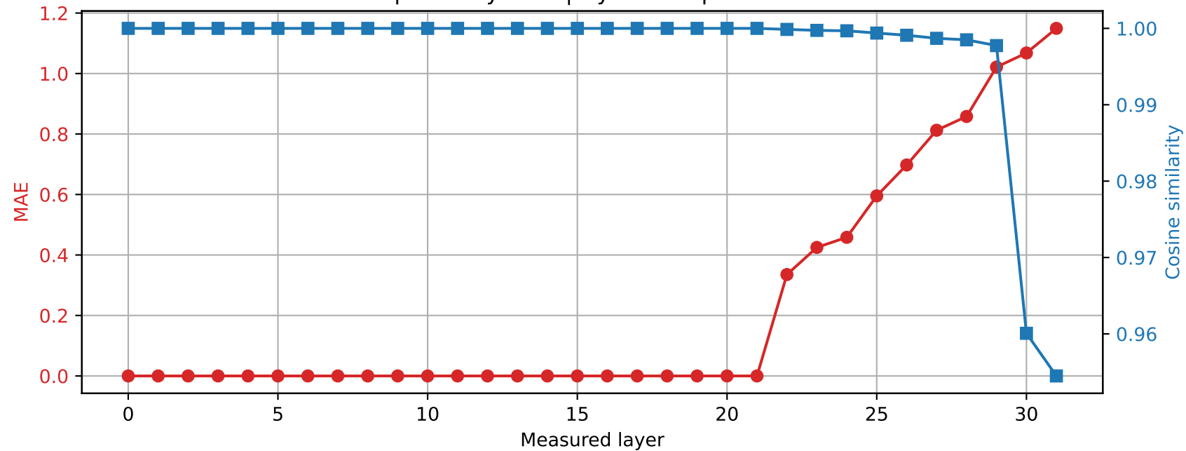
Phi-3-mini-4k-instruct | Prompt 4 Spared layer 21 | Hybrid vs quantized
