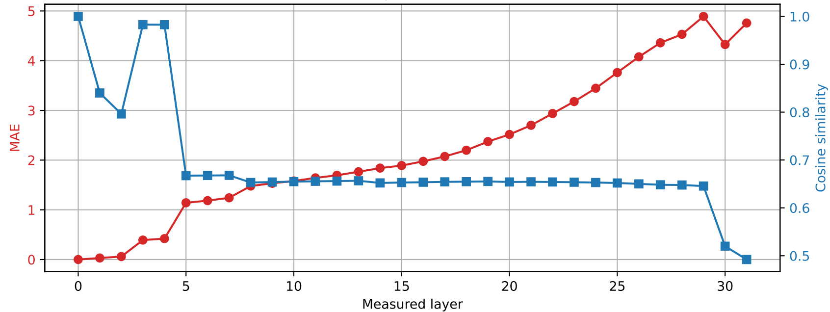
Phi-3-mini-4k-instruct | Prompt 4 Spared layer 22 | Hybrid vs unquantized
