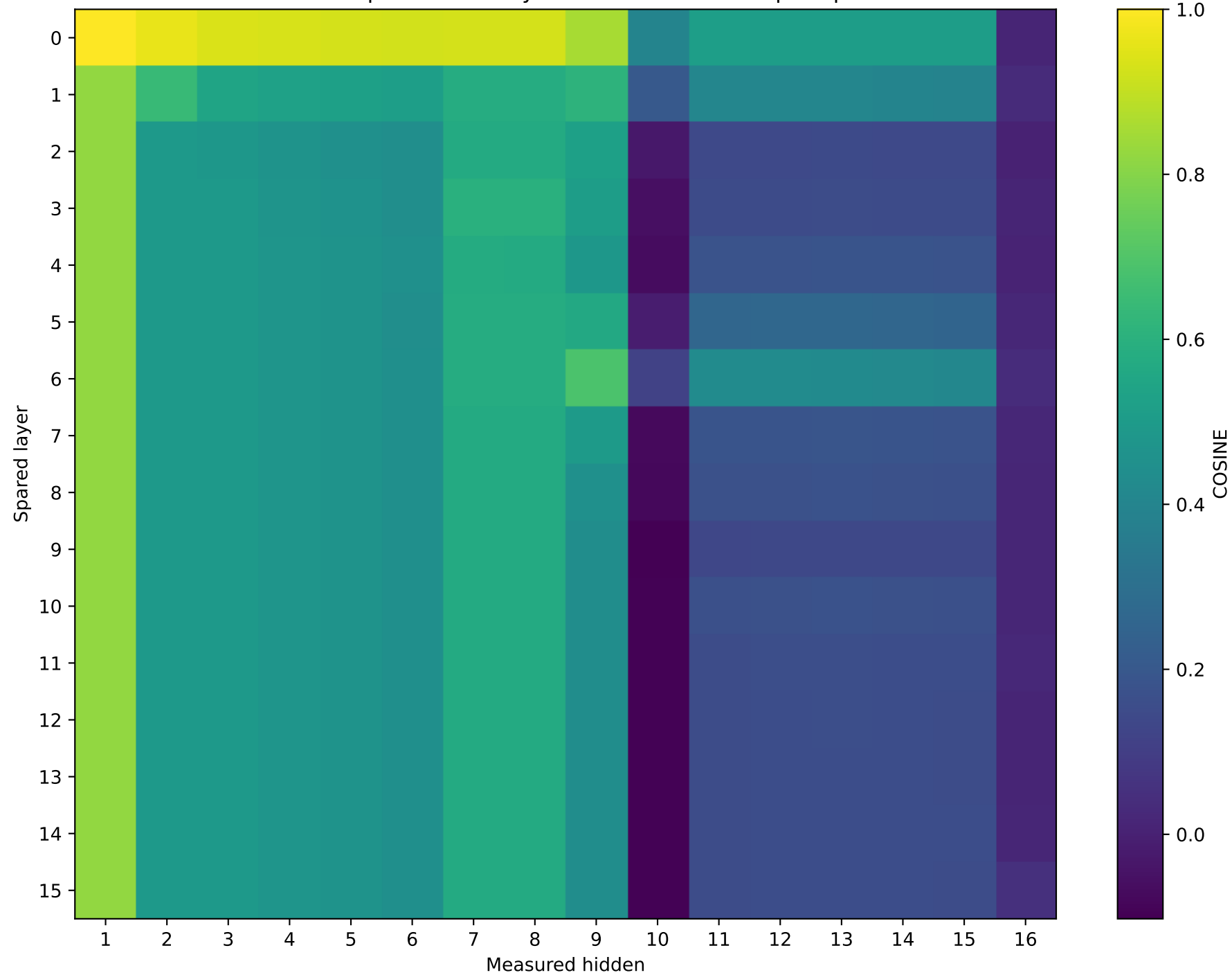
OLMo-1B-hf Mean unquantized vs hybrid cos sim across 5 prompts
