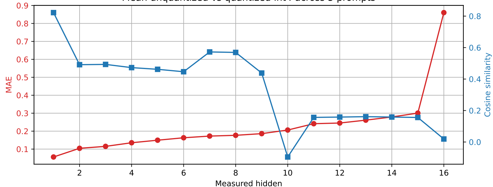
OLMo-1B-hf Mean unquantized vs quantized int4 across 5 prompts
