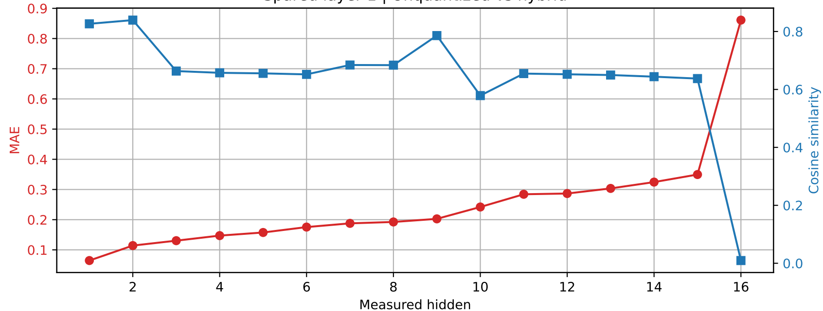
OLMo-1B-hf | Prompt 0 Spared layer 1 | Unquantized vs hybrid
