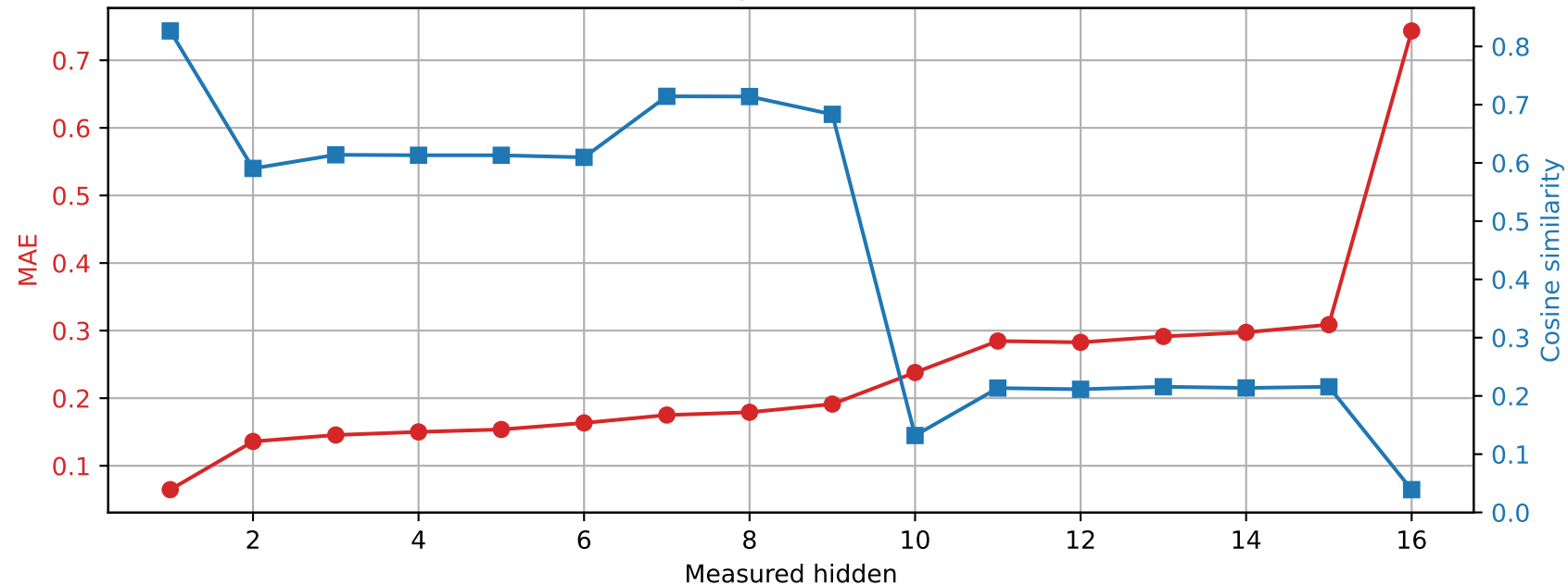
OLMo-1B-hf | Prompt 0 Spared layer 11 | Unquantized vs hybrid
