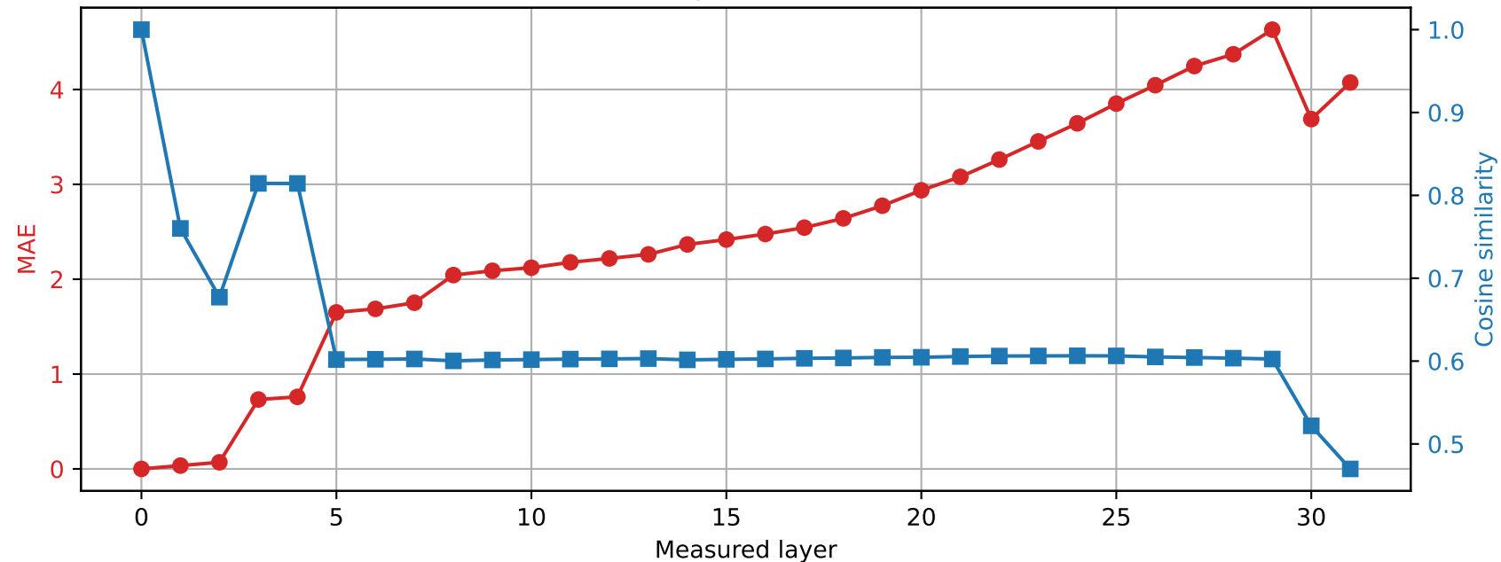
Phi-3-mini-4k-instruct | Prompt 0 Spared layer 19 | Hybrid vs unquantized
