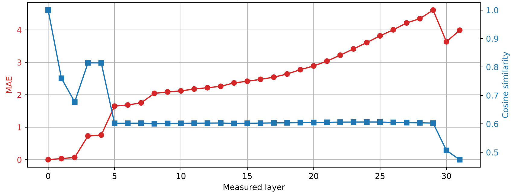
Phi-3-mini-4k-instruct | Prompt 0 Spared layer 21 | Hybrid vs unquantized
