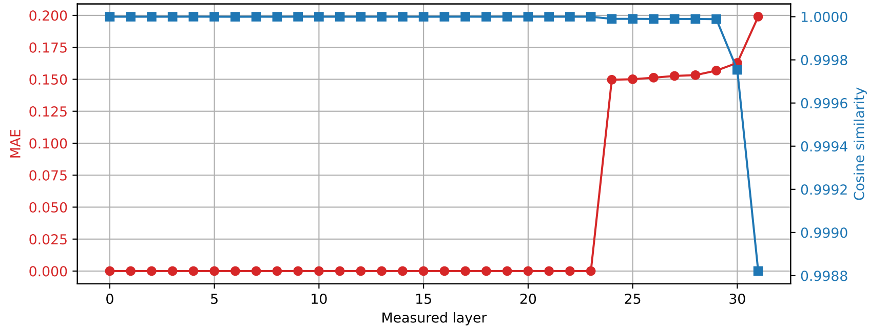
Phi-3-mini-4k-instruct | Prompt 0 Spared layer 23 | Hybrid vs quantized
