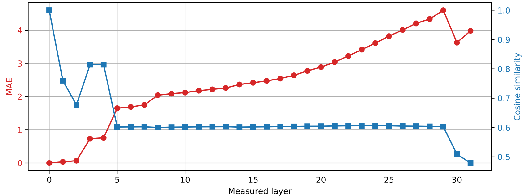
Phi-3-mini-4k-instruct | Prompt 0 Spared layer 26 | Hybrid vs unquantized
