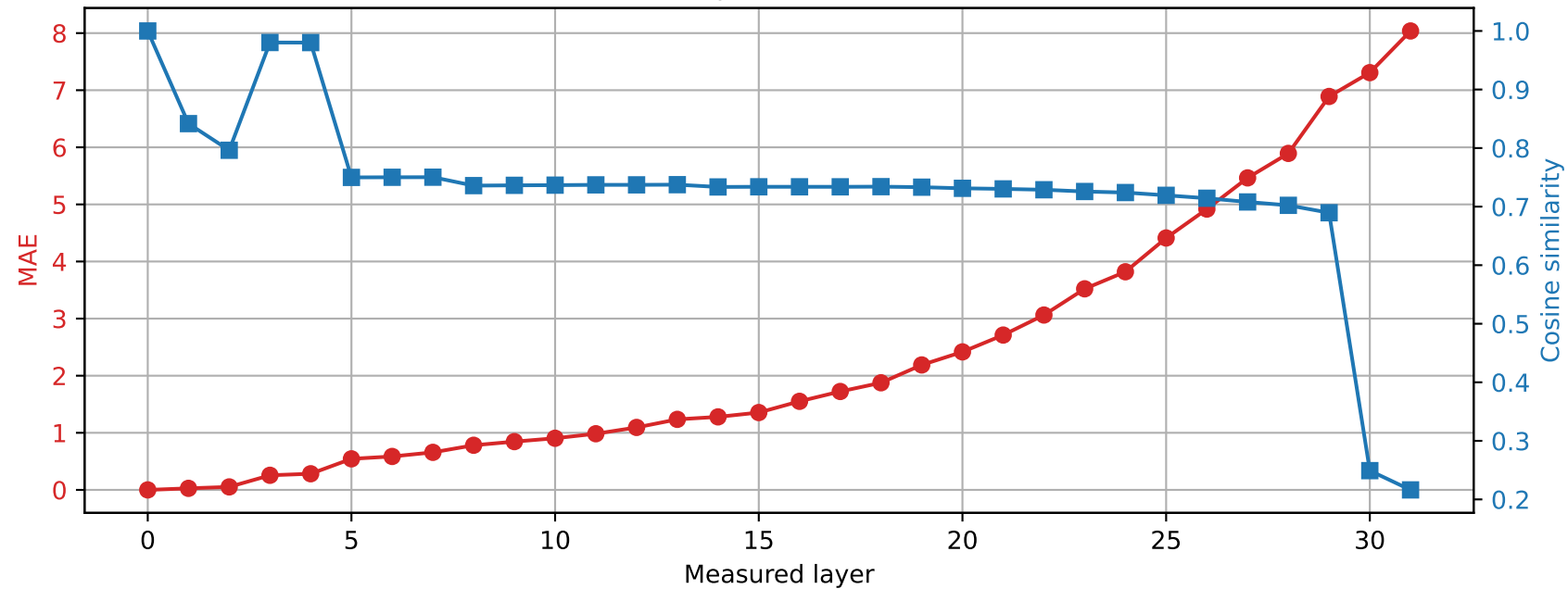
Phi-3-mini-4k-instruct | Prompt 1 Spared layer 1 | Hybrid vs unquantized
