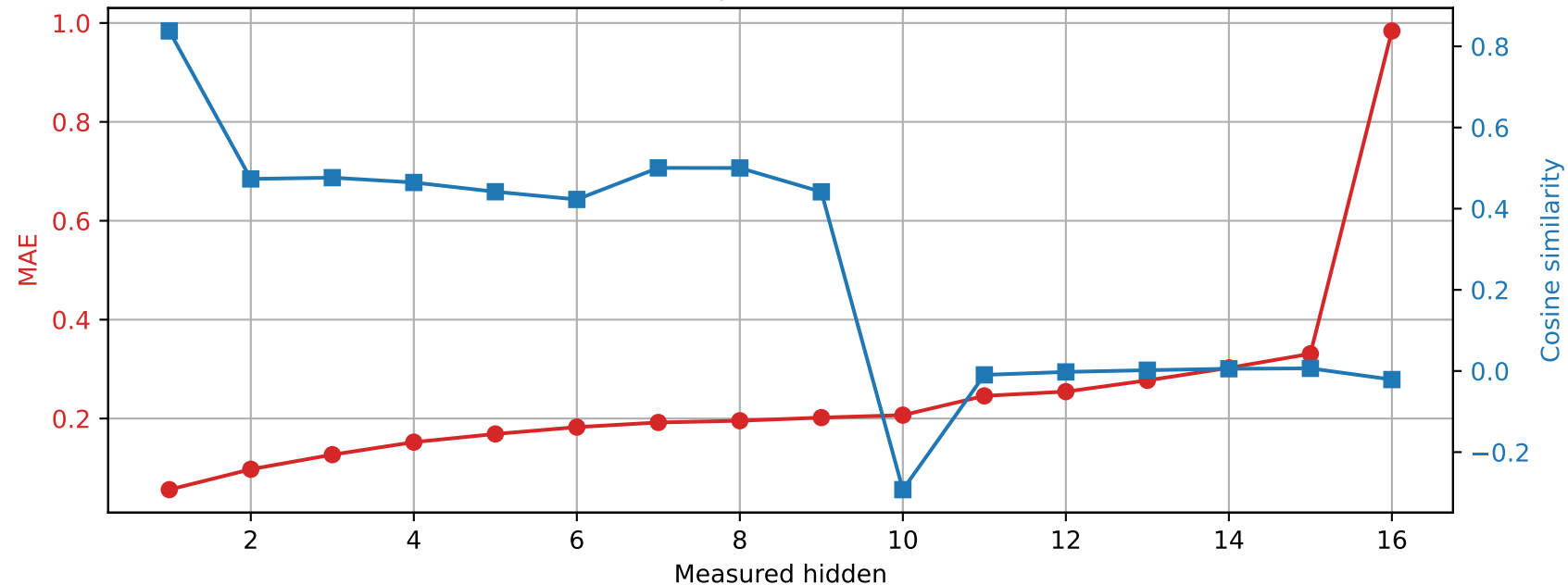
OLMo-1B-hf | Prompt 1 Spared layer 2 | Unquantized vs hybrid
