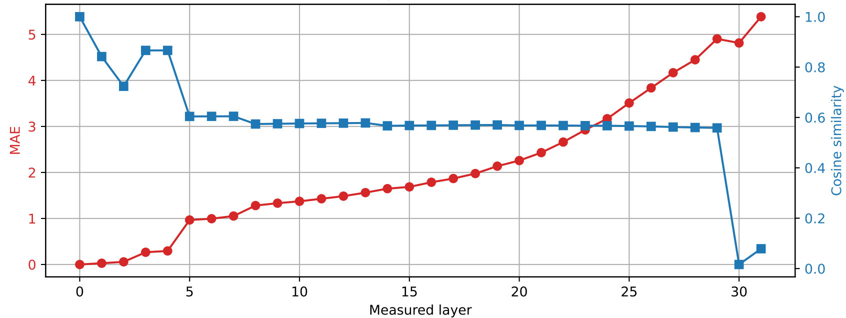
Phi-3-mini-4k-instruct | Prompt 1 Spared layer 4 | Hybrid vs unquantized
