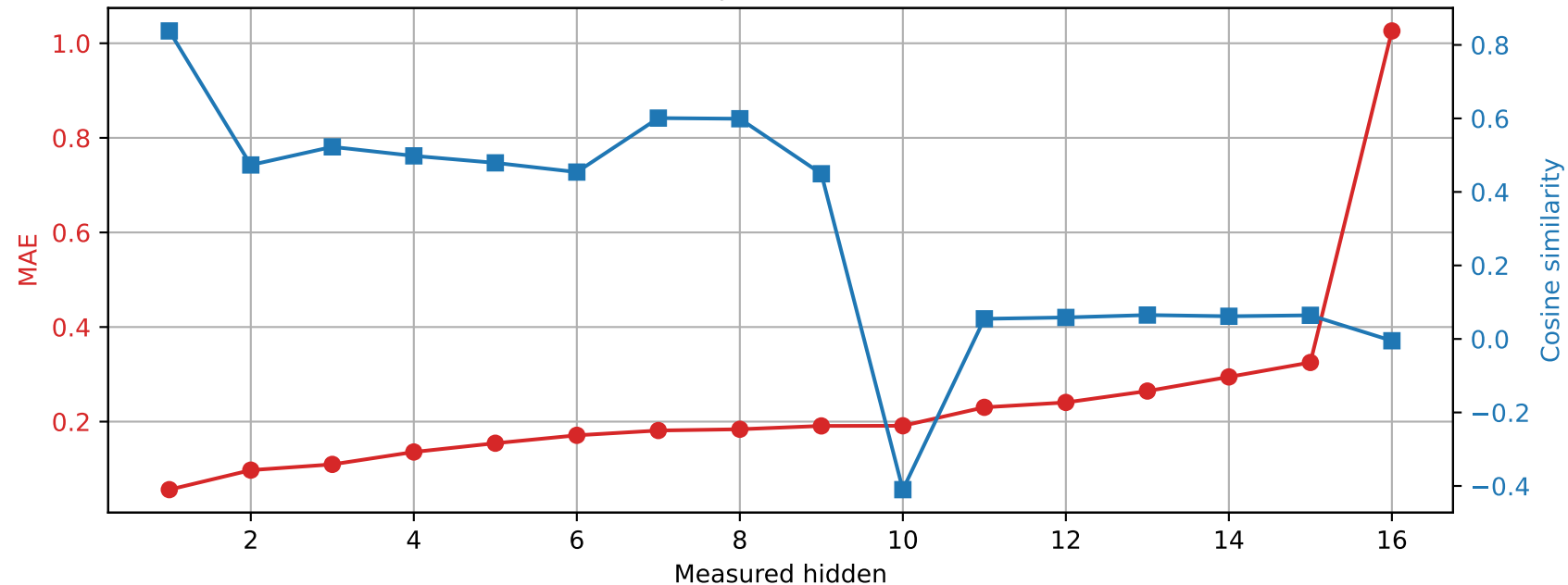
OLMo-1B-hf | Prompt 1 Spared layer 7 | Unquantized vs hybrid
