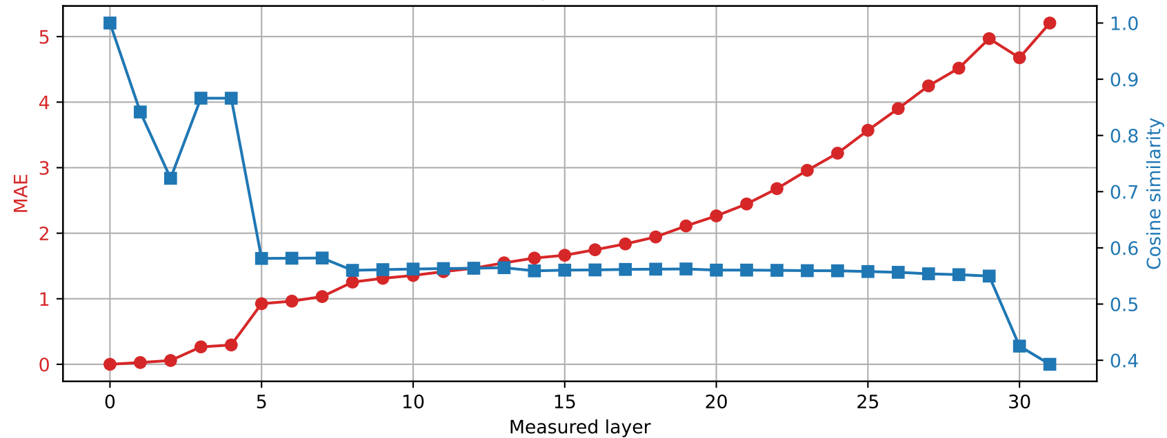
Phi-3-mini-4k-instruct | Prompt 1 Spared layer 12 | Hybrid vs unquantized
