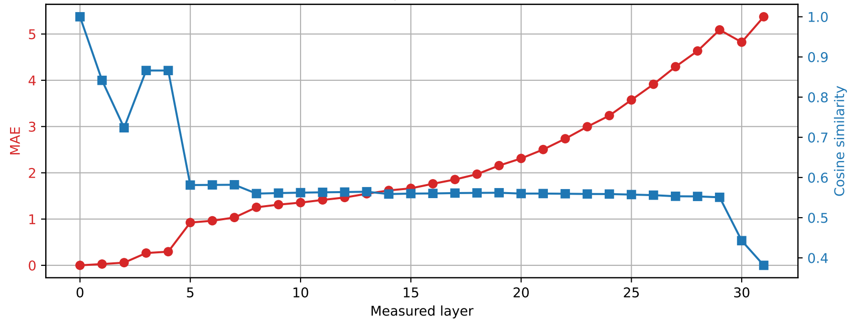
Phi-3-mini-4k-instruct | Prompt 1 Spared layer 27 | Hybrid vs unquantized
