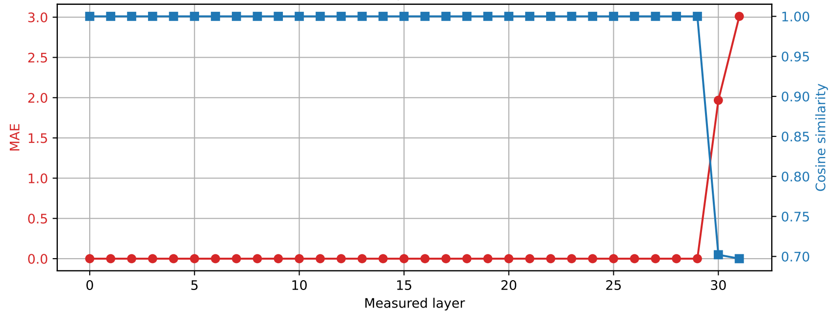
Phi-3-mini-4k-instruct | Prompt 1 Spared layer 29 | Hybrid vs quantized
