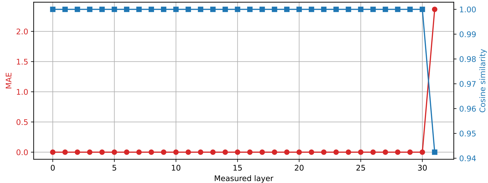
Phi-3-mini-4k-instruct | Prompt 1 Spared layer 30 | Hybrid vs quantized
