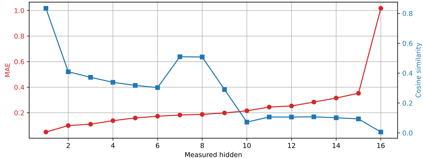
OLMo-1B-hf | Prompt 2 Unquantized vs quantized int4
