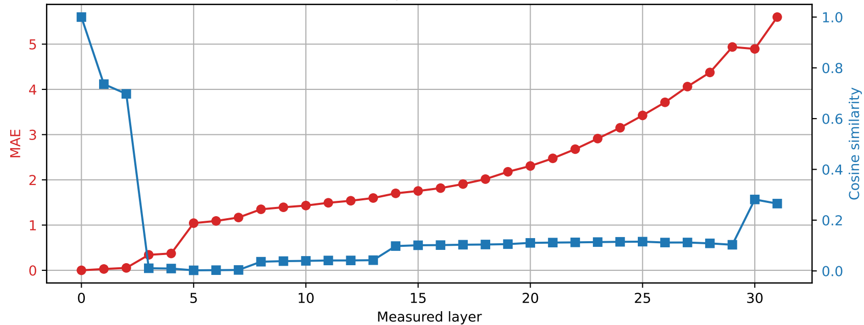
Phi-3-mini-4k-instruct | Prompt 2 Spared layer 2 | Hybrid vs unquantized
