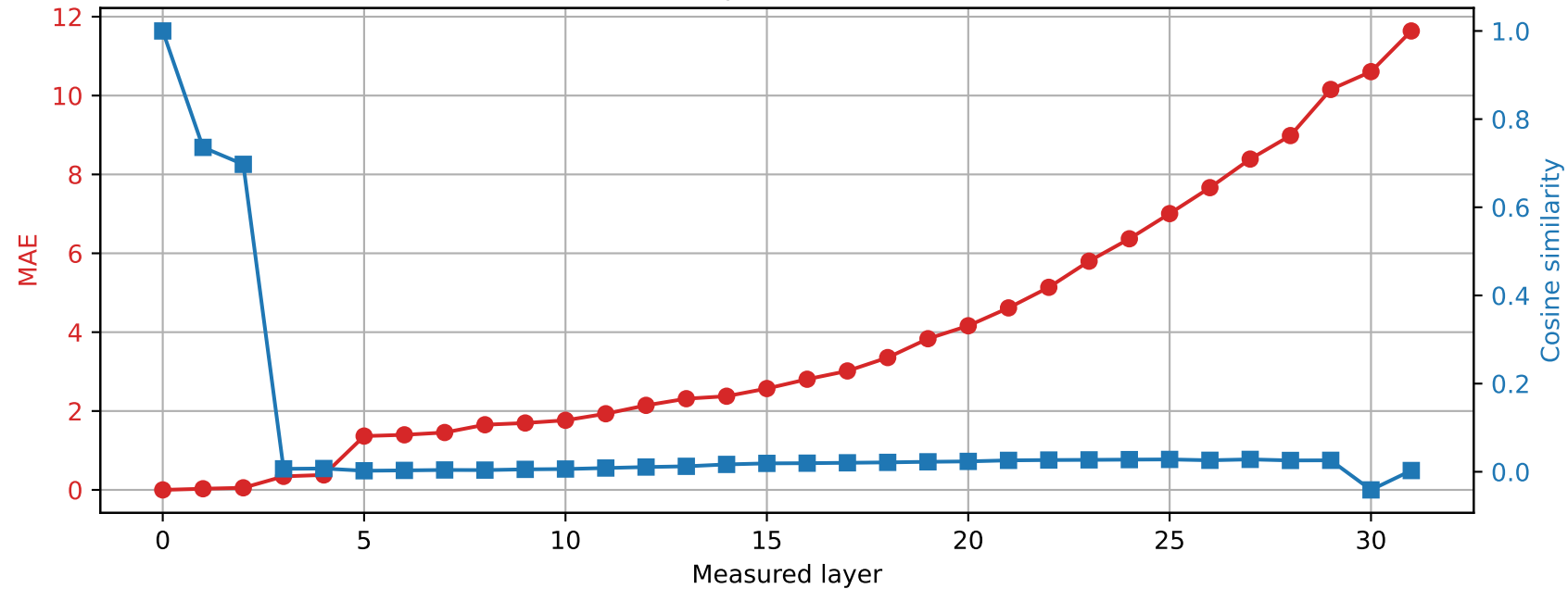
Phi-3-mini-4k-instruct | Prompt 2 Spared layer 4 | Hybrid vs unquantized
