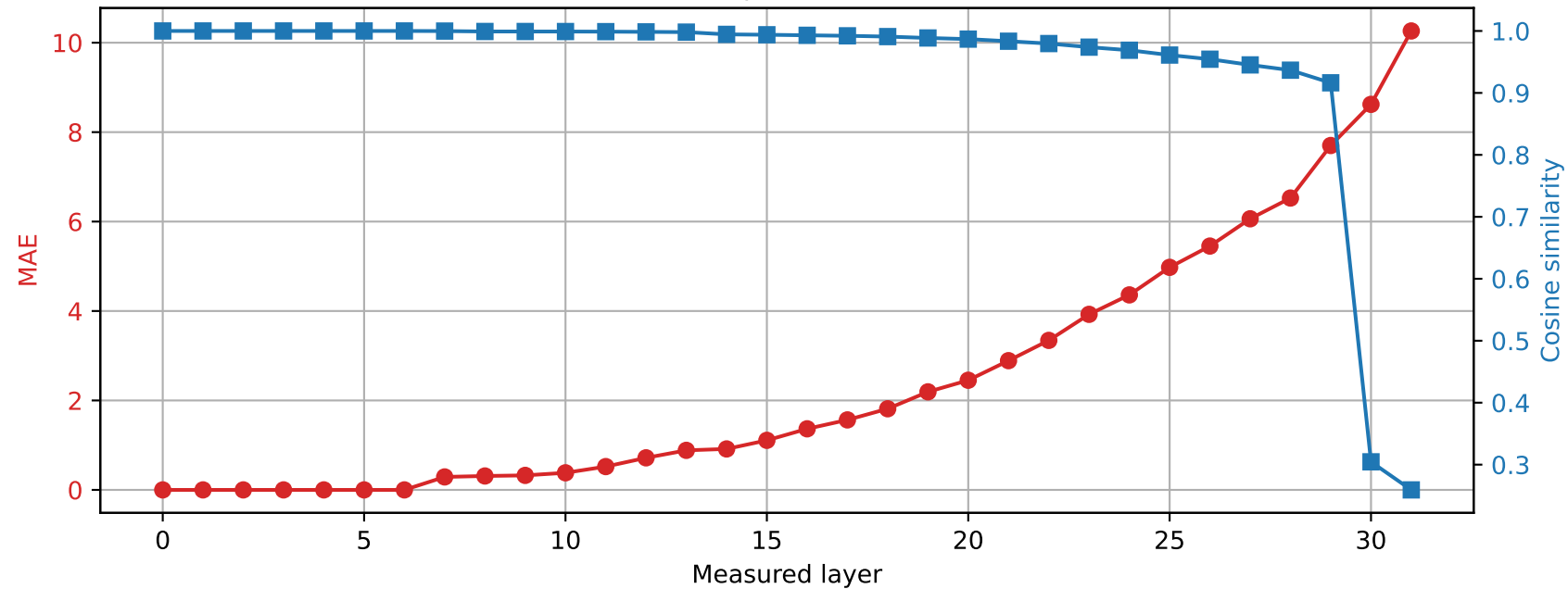
Phi-3-mini-4k-instruct | Prompt 2 Spared layer 6 | Hybrid vs quantized
