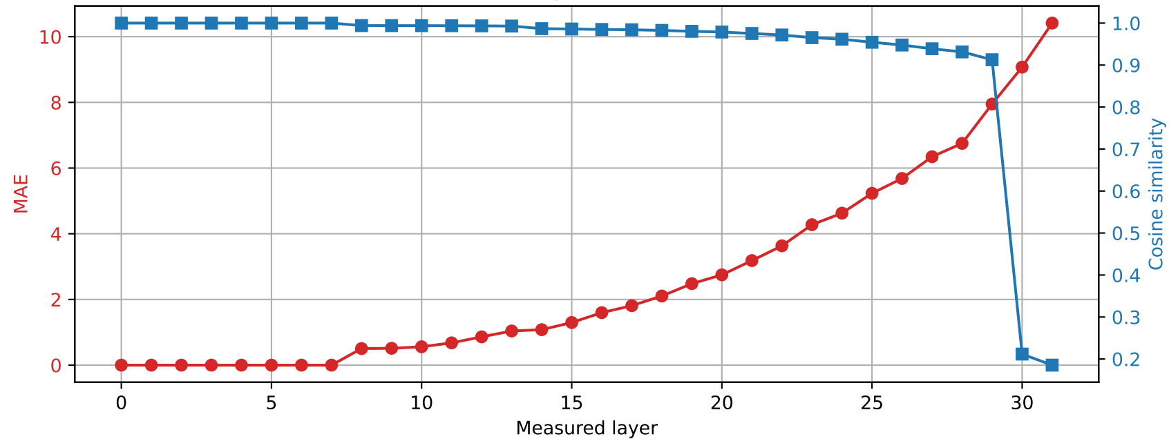
Phi-3-mini-4k-instruct | Prompt 2 Spared layer 7 | Hybrid vs quantized
