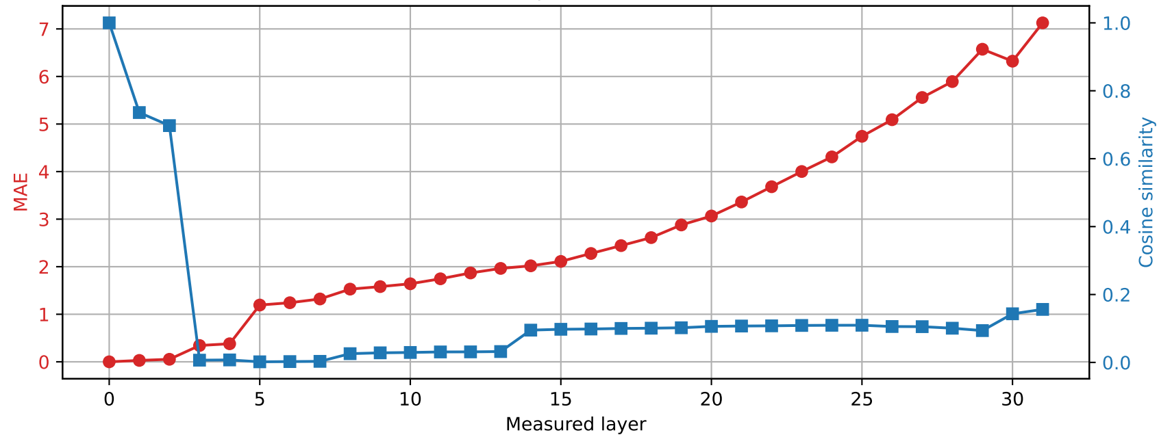
Phi-3-mini-4k-instruct | Prompt 2 Spared layer 22 | Hybrid vs unquantized
