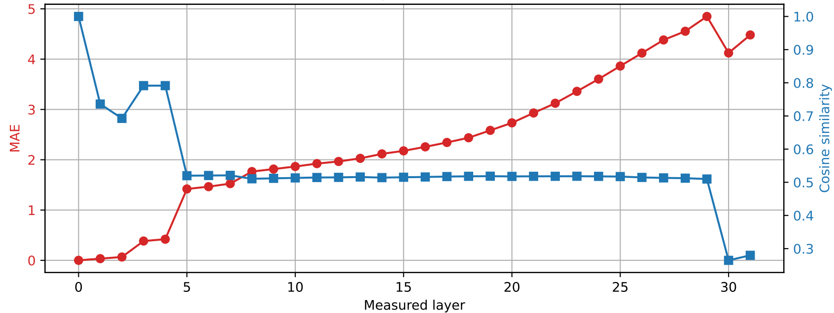
Phi-3-mini-4k-instruct | Prompt 3 Spared layer 2 | Hybrid vs unquantized
