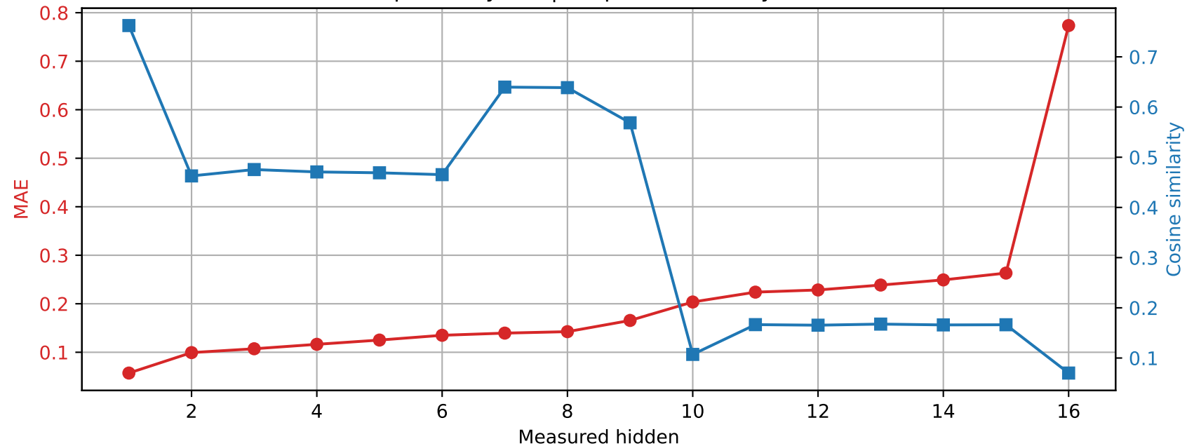
OLMo-1B-hf | Prompt 3 Spared layer 8 | Unquantized vs hybrid
