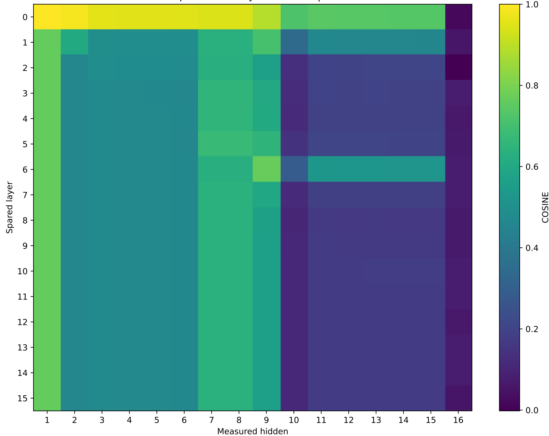
OLMo-1B-hf | Prompt 3 Unquantized vs hybrid cos sim | int4
