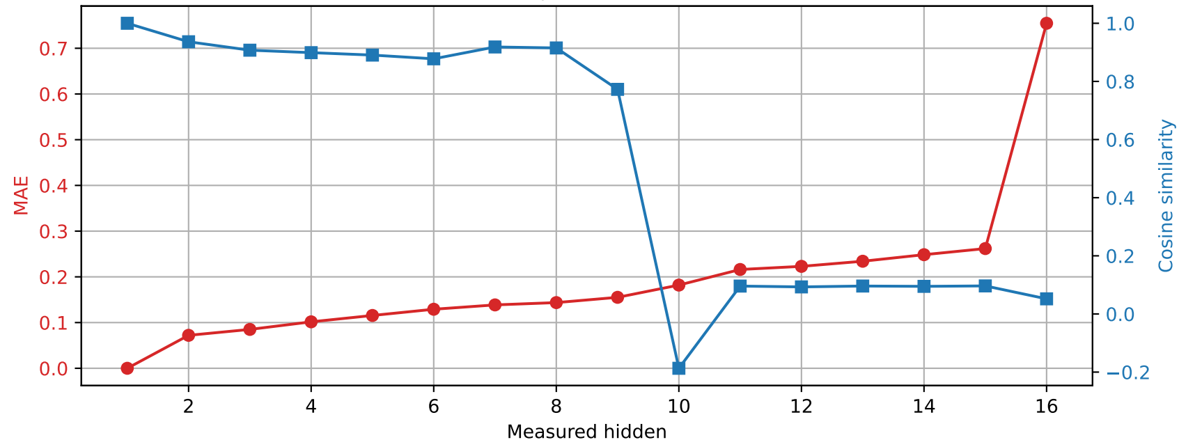
OLMo-1B-hf | Prompt 4 Spared layer 0 | Unquantized vs hybrid
