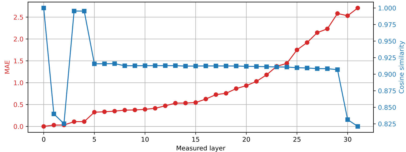
Phi-3-mini-4k-instruct | Prompt 4 Spared layer 0 | Hybrid vs quantized
