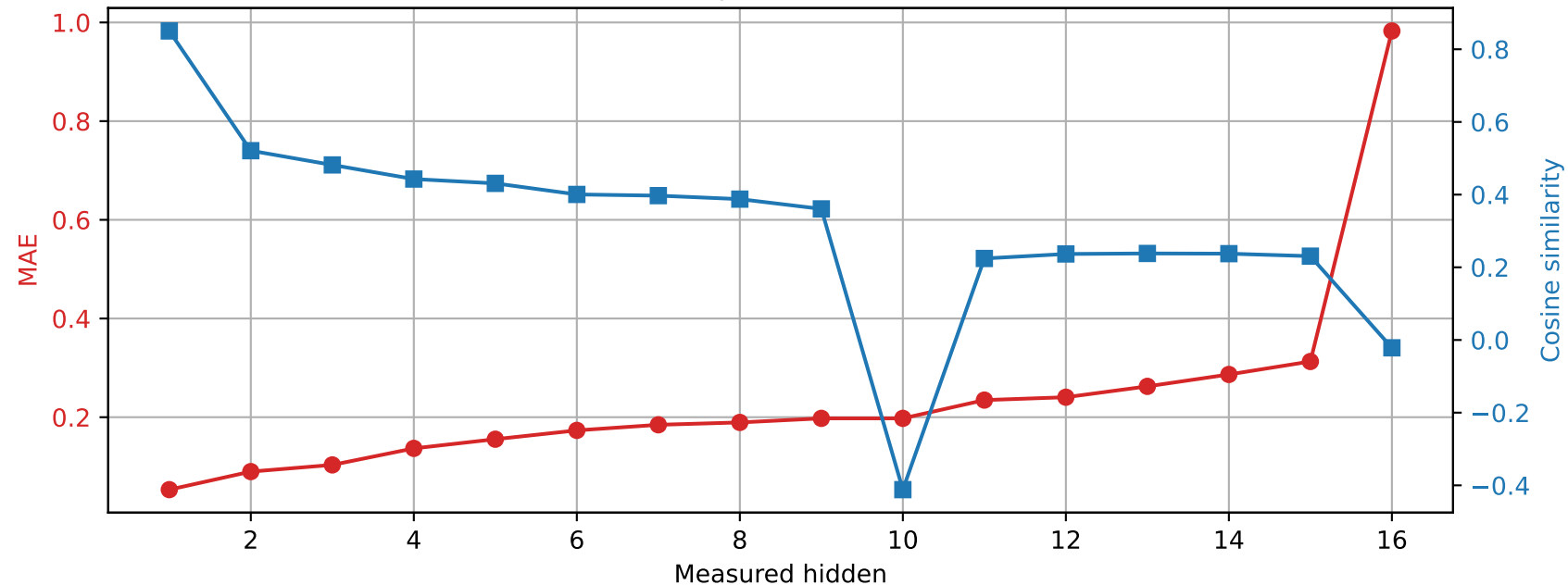
OLMo-1B-hf | Prompt 4 Spared layer 7 | Unquantized vs hybrid
