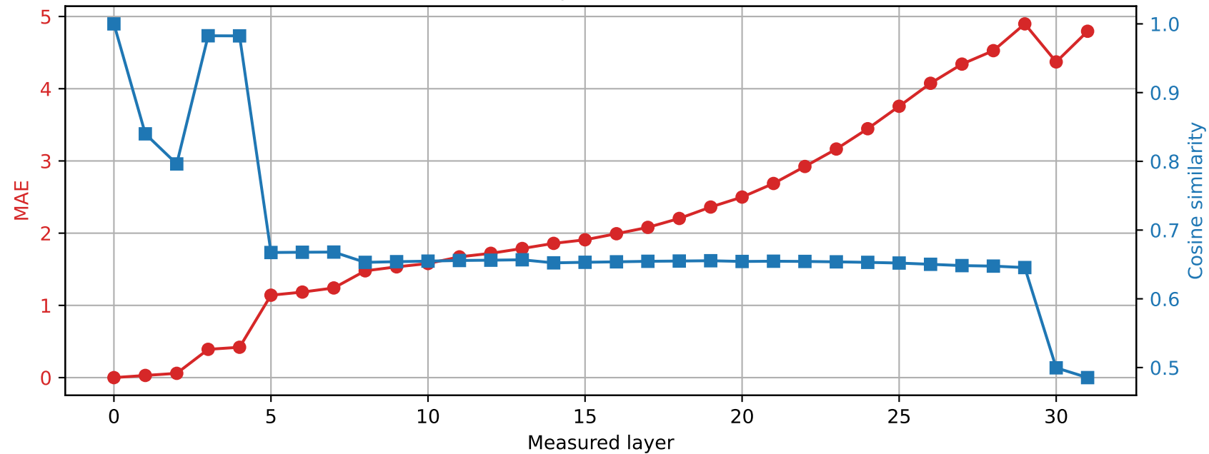
Phi-3-mini-4k-instruct | Prompt 4 Spared layer 10 | Hybrid vs unquantized
