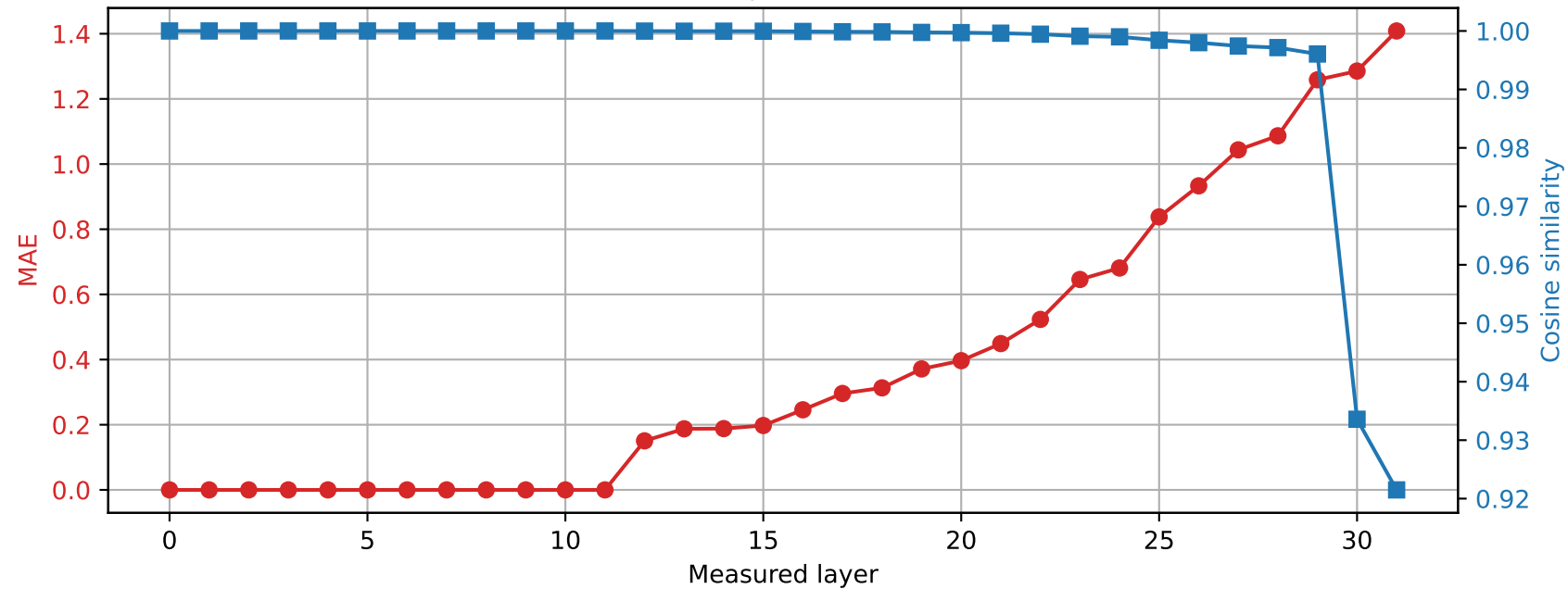
Phi-3-mini-4k-instruct | Prompt 4 Spared layer 11 | Hybrid vs quantized
