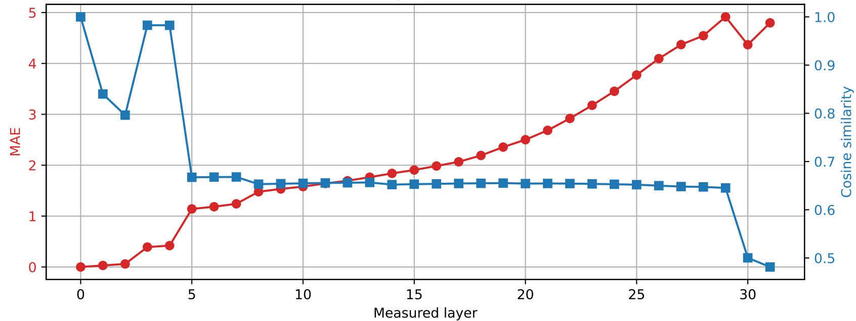
Phi-3-mini-4k-instruct | Prompt 4 Spared layer 14 | Hybrid vs unquantized
