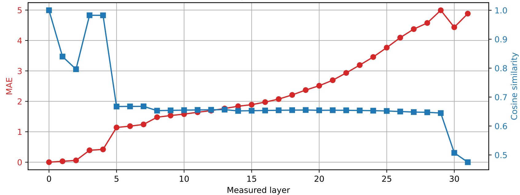
Phi-3-mini-4k-instruct | Prompt 4 Spared layer 17 | Hybrid vs unquantized
