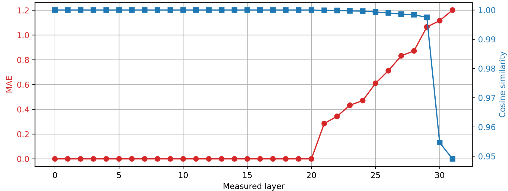
Phi-3-mini-4k-instruct | Prompt 4 Spared layer 20 | Hybrid vs quantized
