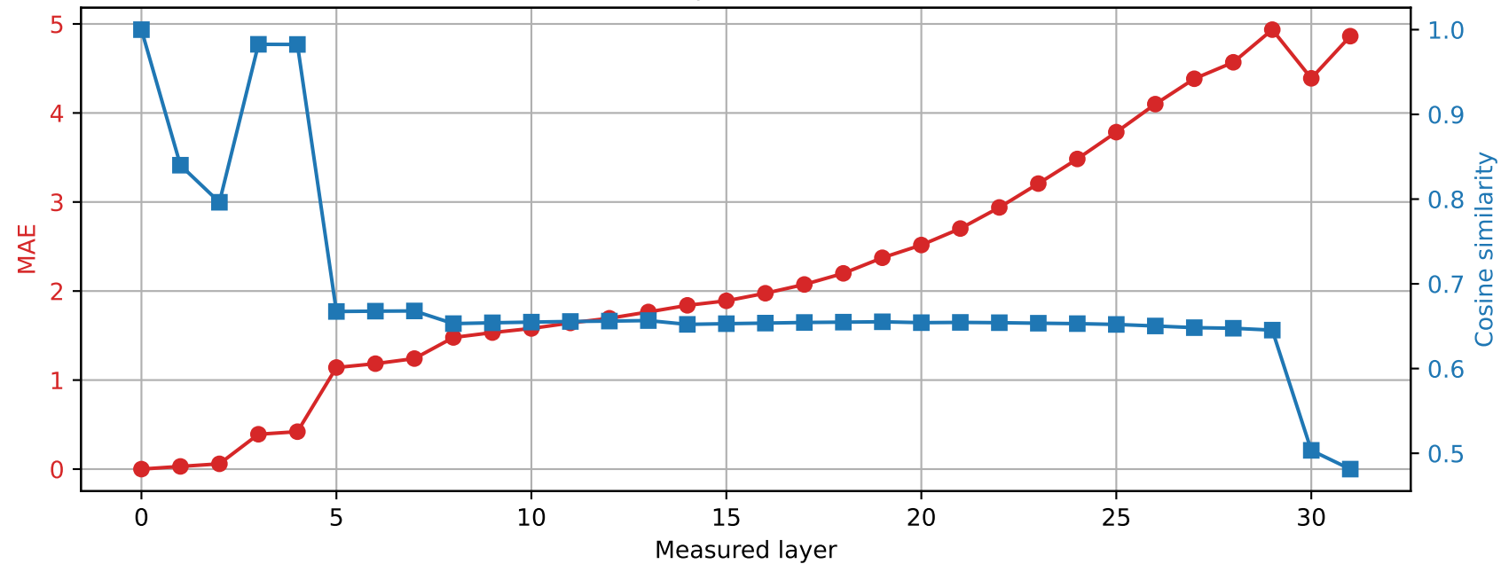
Phi-3-mini-4k-instruct | Prompt 4 Spared layer 23 | Hybrid vs unquantized
