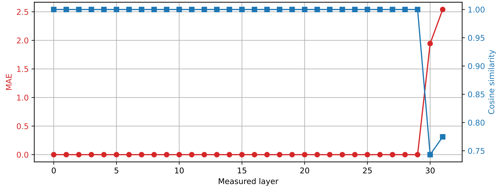
Phi-3-mini-4k-instruct | Prompt 4 Spared layer 29 | Hybrid vs quantized
