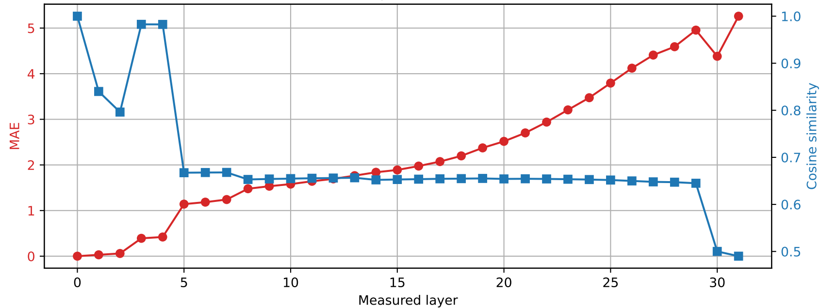
Phi-3-mini-4k-instruct | Prompt 4 Spared layer 30 | Hybrid vs unquantized
