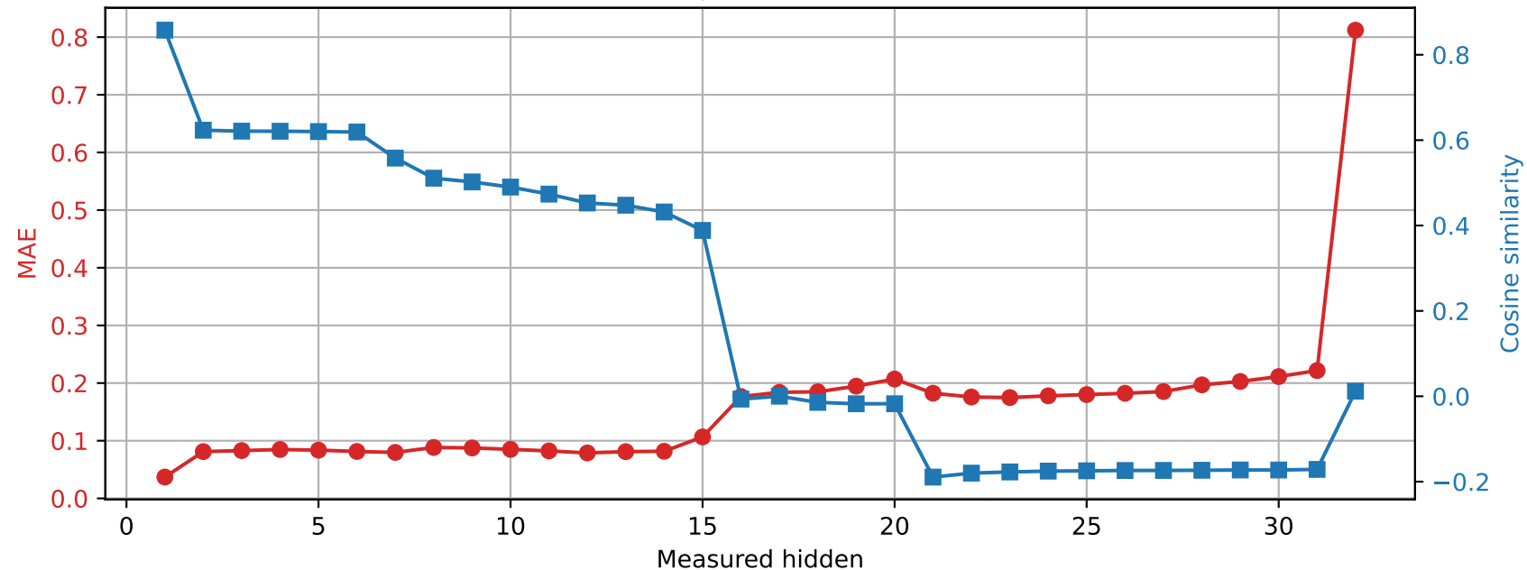
OLMo-7B-hf | Prompt 0 Spared layer 4 | Unquantized vs hybrid
