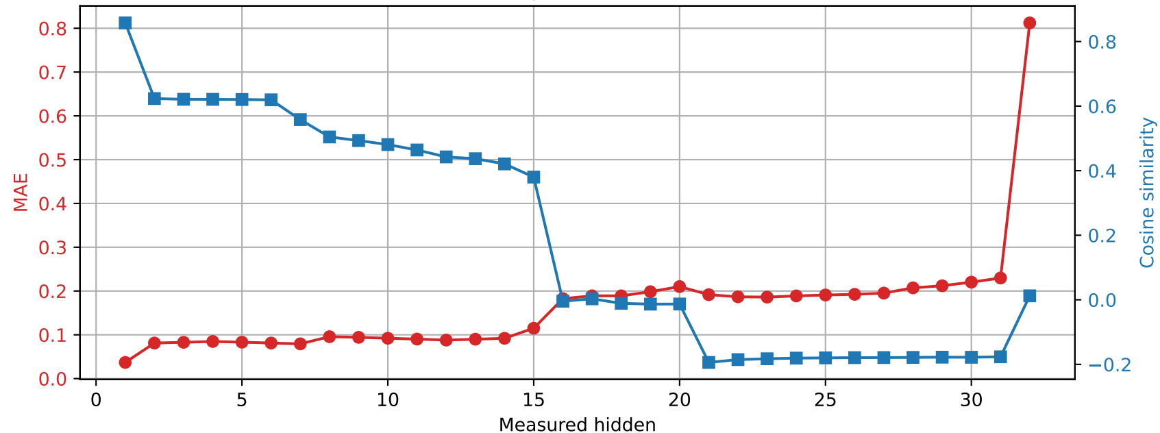
OLMo-7B-hf | Prompt 0 Spared layer 7 | Unquantized vs hybrid
