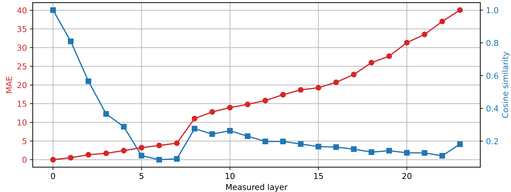
SmolLM2-1.7B-Instruct | Prompt 0 Spared layer 8 | Hybrid vs unquantized
