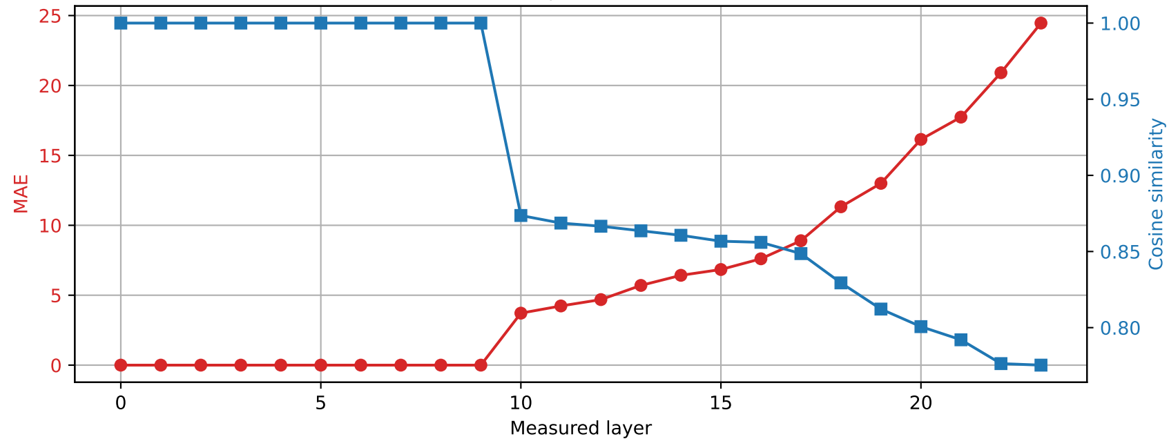
SmolLM2-1.7B-Instruct | Prompt 0 Spared layer 9 | Hybrid vs quantized
