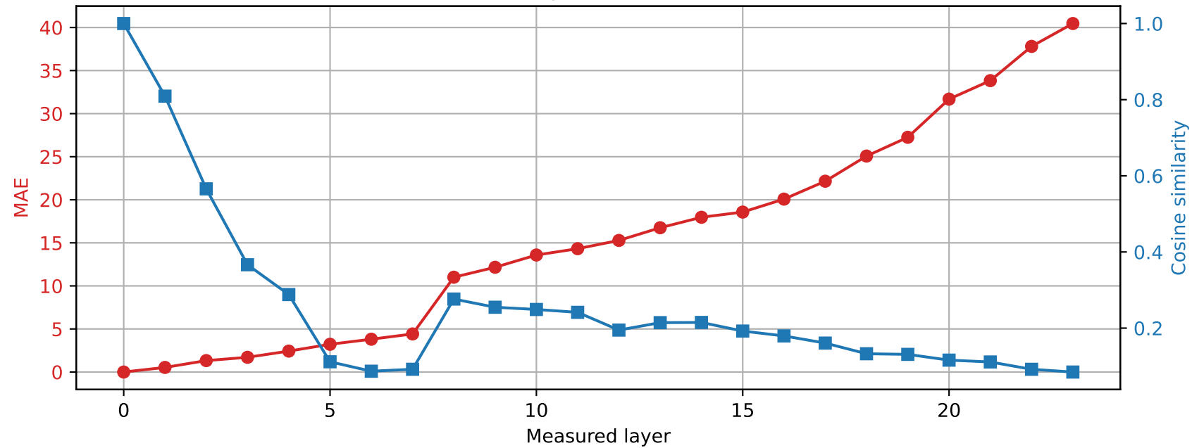
SmolLM2-1.7B-Instruct | Prompt 0 Spared layer 9 | Hybrid vs unquantized
