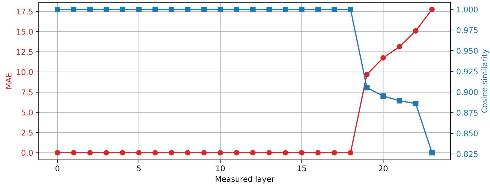
SmolLM2-1.7B-Instruct | Prompt 0 Spared layer 18 | Hybrid vs quantized
