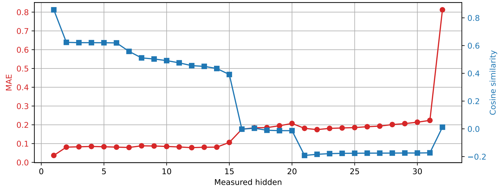
OLMo-7B-hf | Prompt 0 Spared layer 22 | Unquantized vs hybrid
