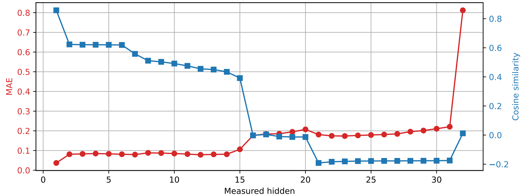
OLMo-7B-hf | Prompt 0 Spared layer 29 | Unquantized vs hybrid
