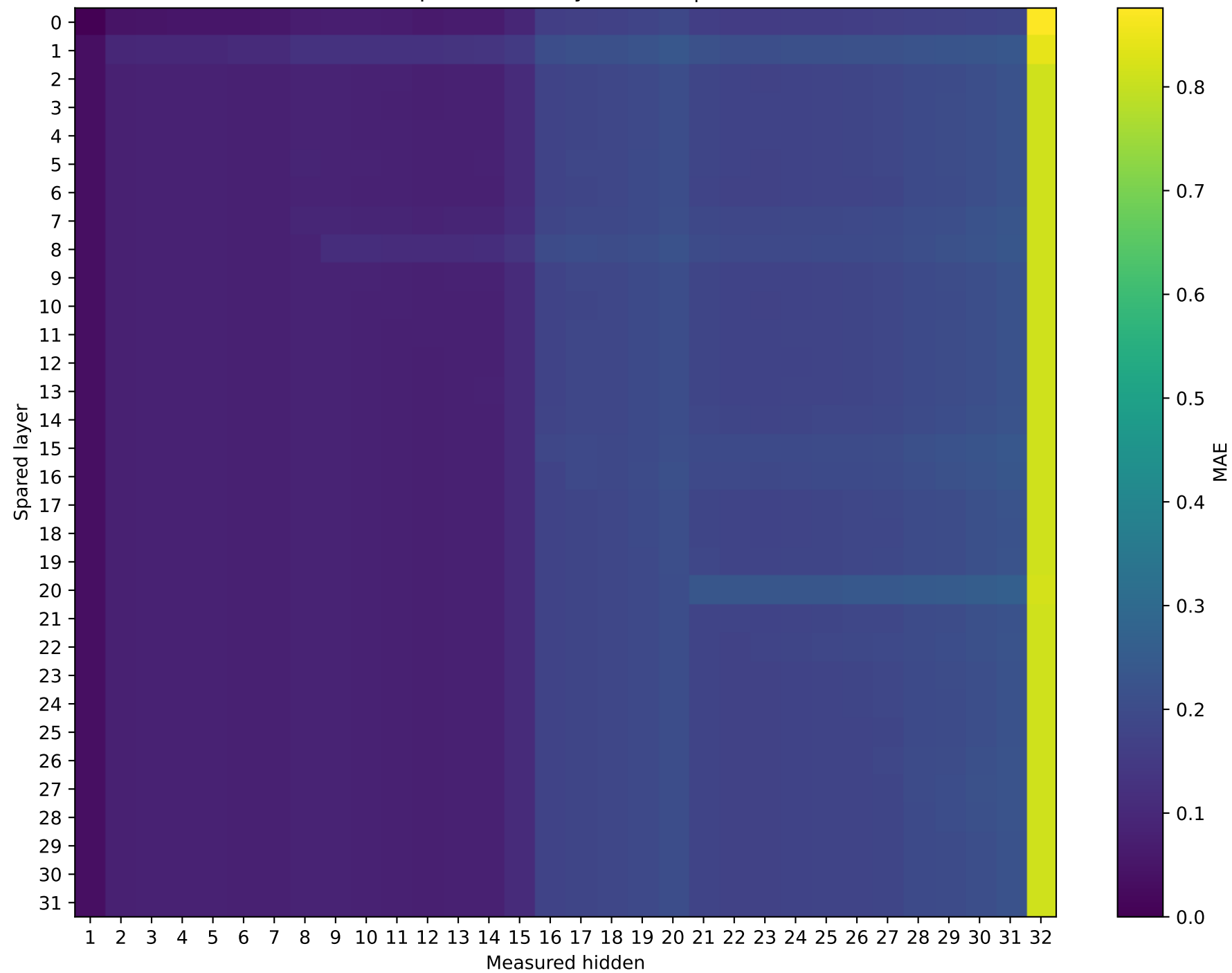
OLMo-7B-hf | Prompt 0 Unquantized vs hybrid MAE | int4
