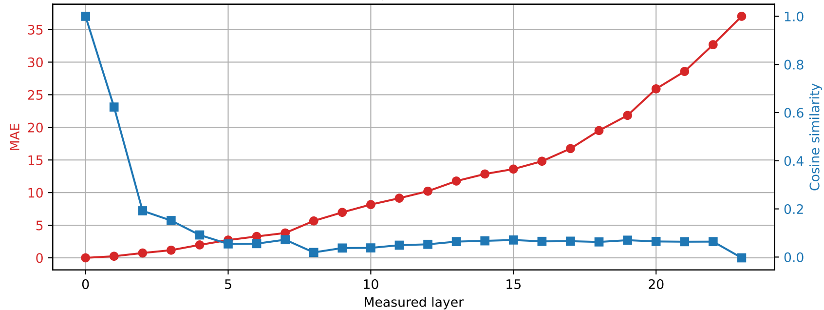
SmolLM2-1.7B-Instruct | Prompt 1 Spared layer 2 | Hybrid vs unquantized
