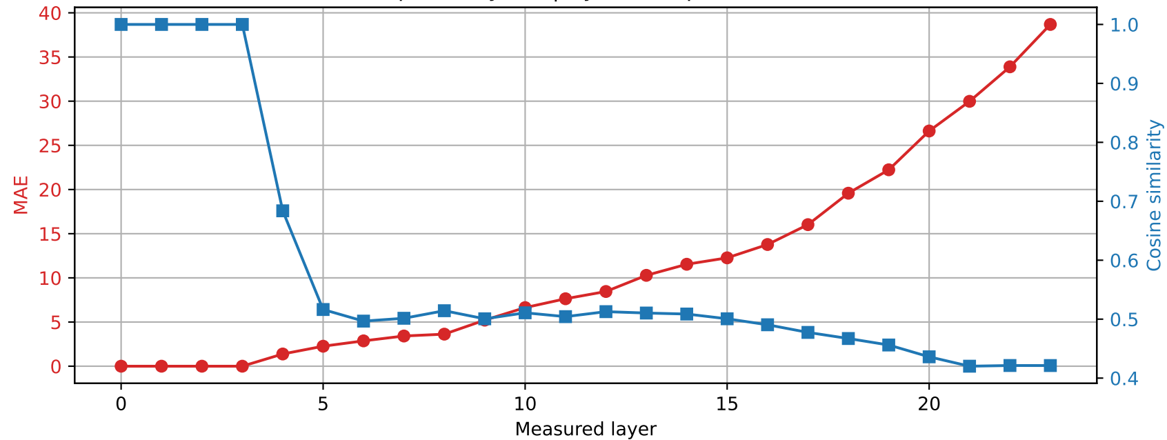
SmolLM2-1.7B-Instruct | Prompt 1 Spared layer 3 | Hybrid vs quantized
