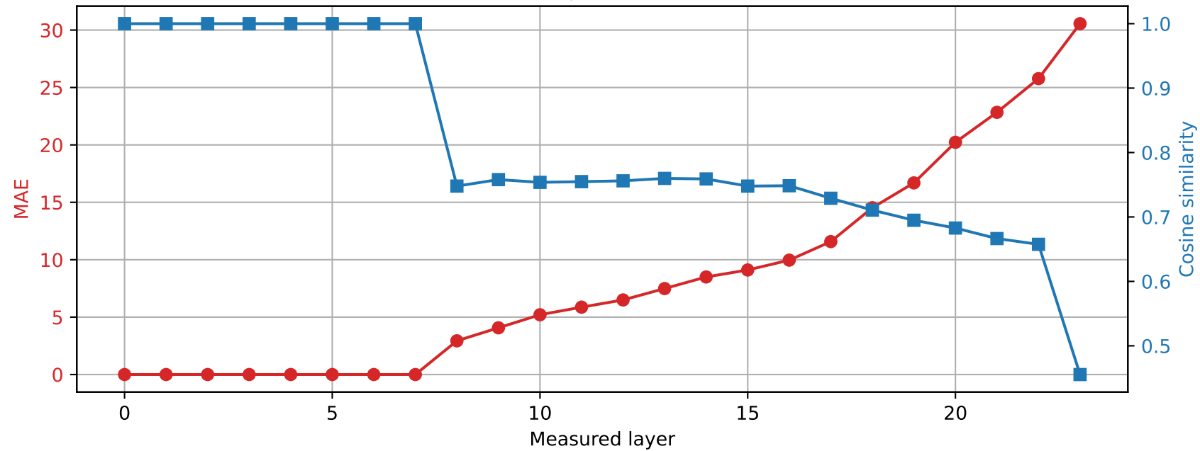
SmolLM2-1.7B-Instruct | Prompt 1 Spared layer 7 | Hybrid vs quantized
